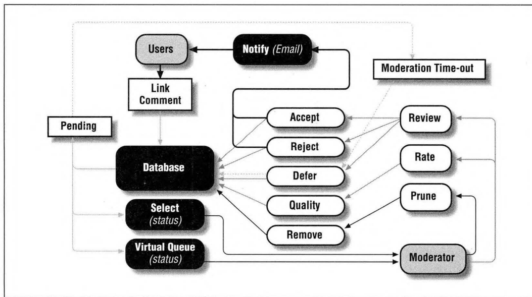
Figure 8: Moderation Work Flow
